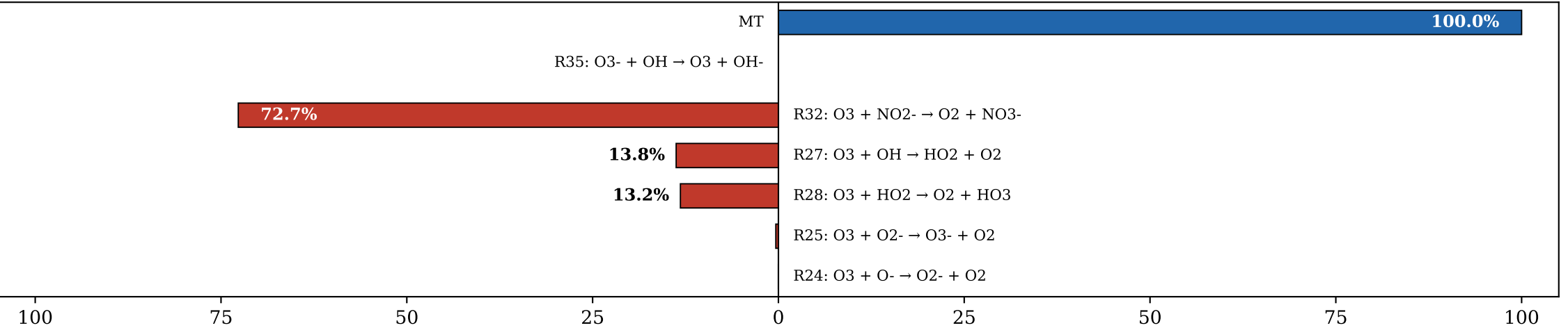
(c) NO 2 - (Σsrc = 4.50e-08 M/s)
